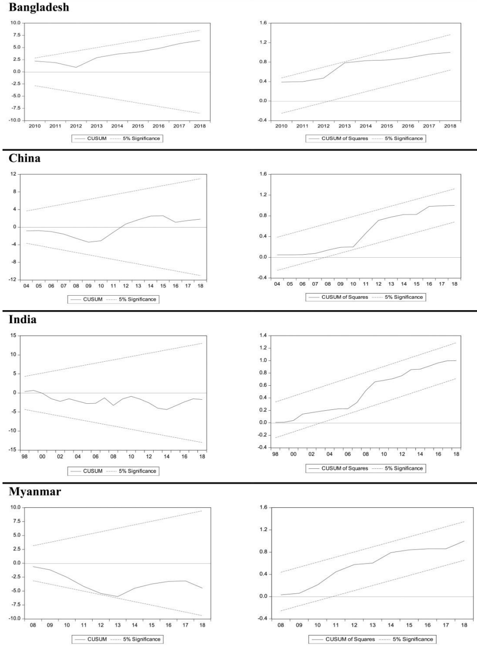
Fig. 5: CUSUM and CUSUM of square tests
